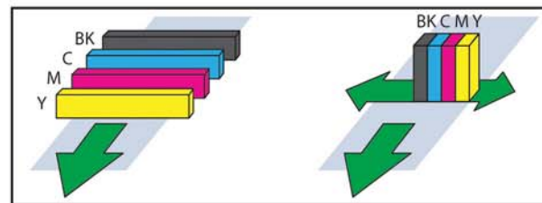
Single-pass printing (SCC-4000D)
